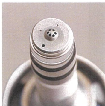
EURO-6 Delphi Multec® GDi Multi-Hole
